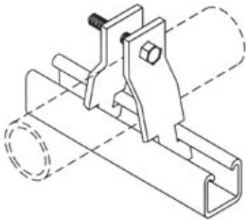
"Non-Metallic" Universal Pipe Clamps
