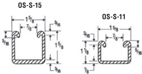
Single Strut
