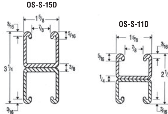
Double Strut "Back to Back" Strut
